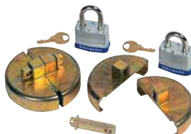
08510 steel model fits DN20 and DN50 bung with set of 2 padlocks
